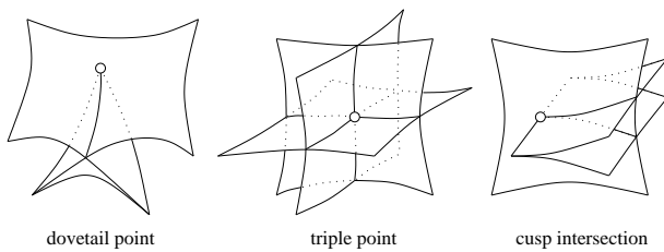
Figure 5: Left: a portion of the pedal surface in which a self-intersection and two cusps end at a dovetail point. Middle: three sheets of the pedal surface intersecting in a triple point. Right: a cusp intersecting another sheet of the pedal surface.
