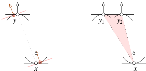
Figure 9: A one-legged configuration on the left and a two-legged configuration on the right. In both configurations, we can increase the height difference by tilting the normal direction towards the left.
