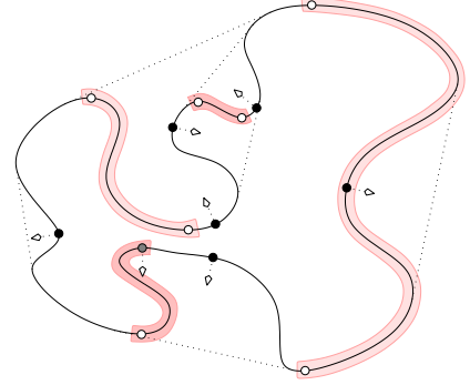
Figure 3: A 1-manifold with marked (white and shaded) critical points of the vertical height function. The shaded strips along the curve connect paired critical points. The black and shaded dots mark two- and one-legged elevation maxima.
