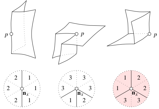
Figure 8: Top row: the three sheets of \mathbb{Q} after [possible ways] of cutting and gluing the neighborhood of a triple point p in \mathbb{P} . Bottom row: the corresponding pairing patterns in the neighborhood of \mathbf{n}_x , each belonging to one of the three points paired with the three feet. The (shaded) Mercedes star is necessary for a three-legged maximum.
