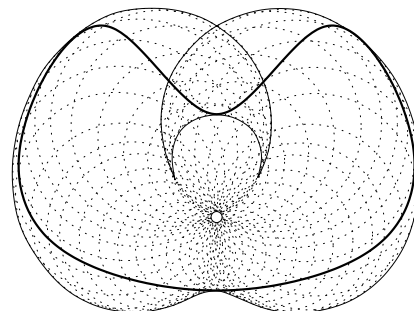
Figure 4: A smoothly embedded (boldface solid) closed curve and the (solid) image of the pedal function constructed as the evolute of the (dotted) diameter circles between the curve and the origin.
